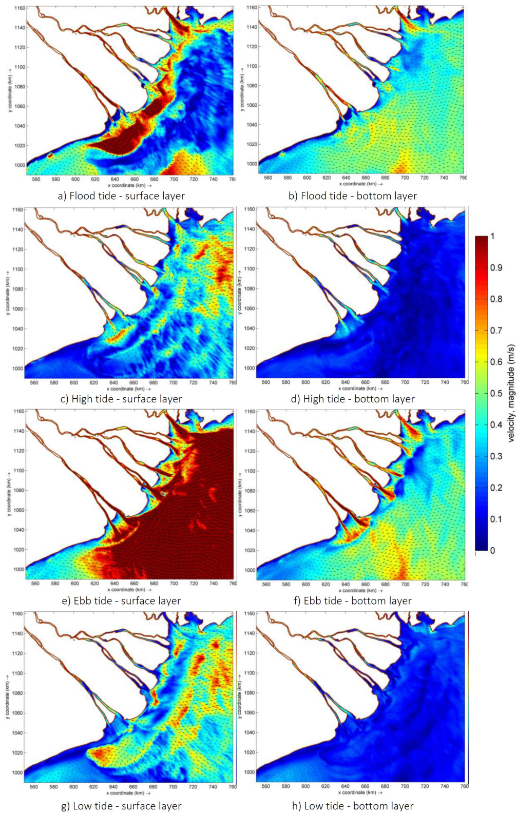
Figure 6. Current velocity during (m/s) the spring tide in May 2019
