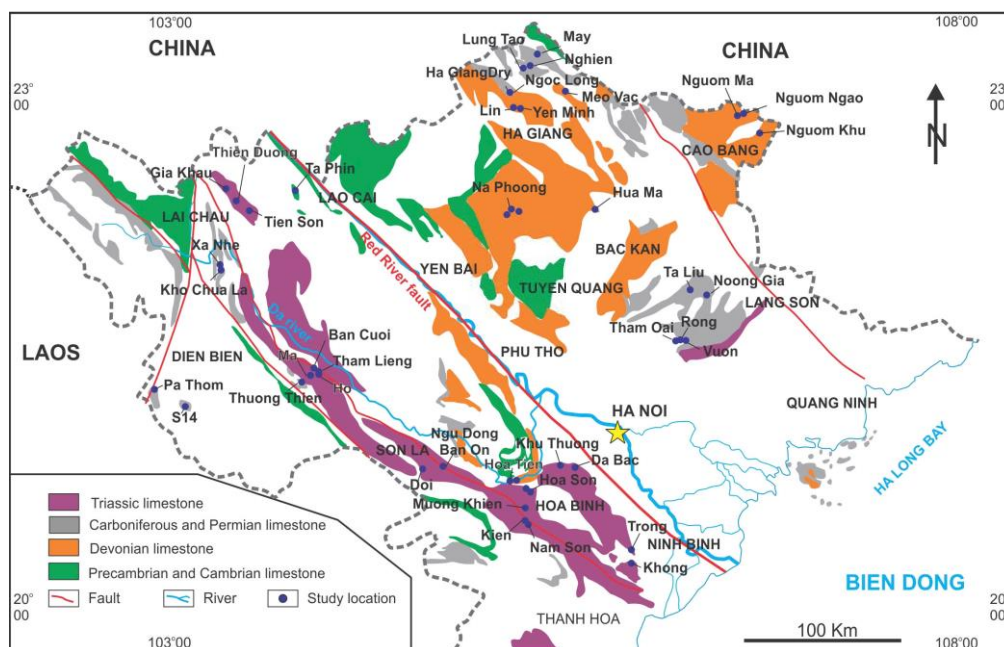
Figure 1. Distribution map of carbonate formations in Northern Vietnam and locations of surveyed caves in this study (The Department of Geology and Minerals of Vietnam, 2005; Phan et al., 1991).
