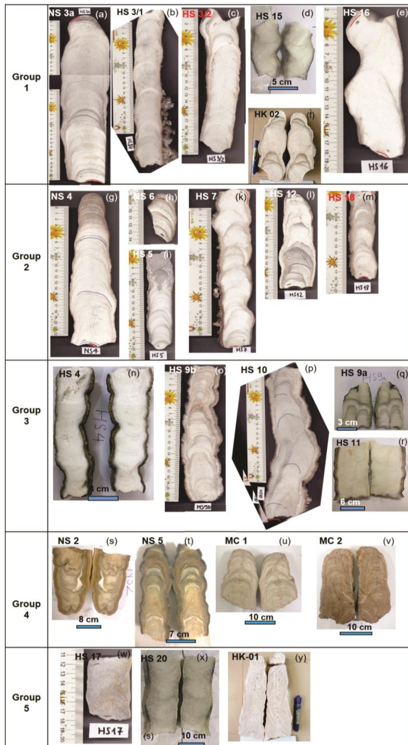
Figure 6. Classification of stalagmites in some selected caves into 5 groups
