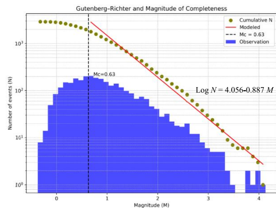
Figure 8. Magnitude of completeness ( M_c ) estimated using the Gutenberg-Richter relation
