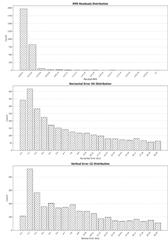
Figure S1. Lateral error and RMS distribution results from NonLinLoc Processing
