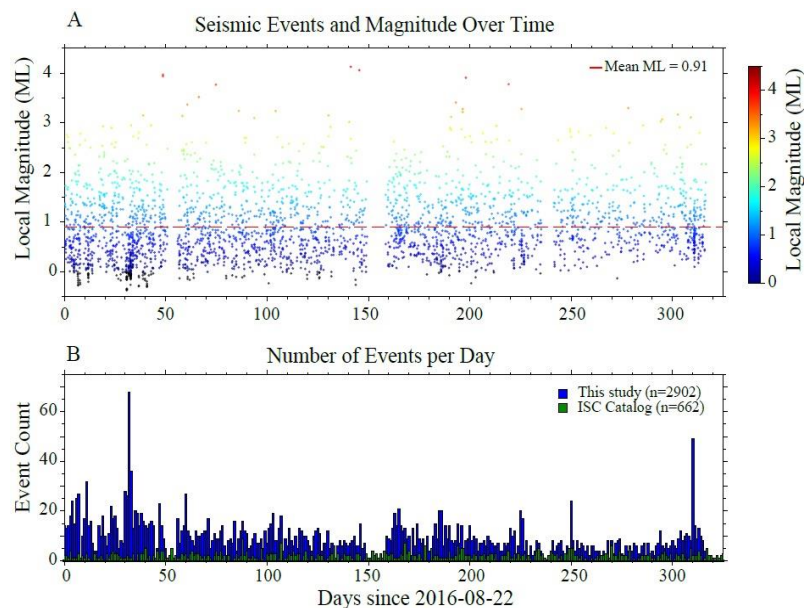
Figure 6. (A) Magnitude variation of seismic events; (B) Daily variation of earthquake occurrences
