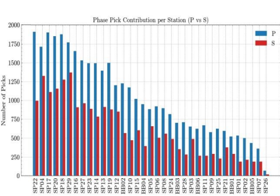
Figure S3. Number of associated phase picks (P and S) and associated earthquake events contributed by each seismic station
