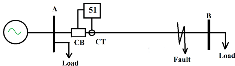
Figure 6. One phase diagram of a transmission system.
