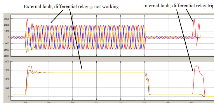
Figure 15. Instantaneous waveform and RMS waveform of short-circuit current in the case of Differential relay protection.
