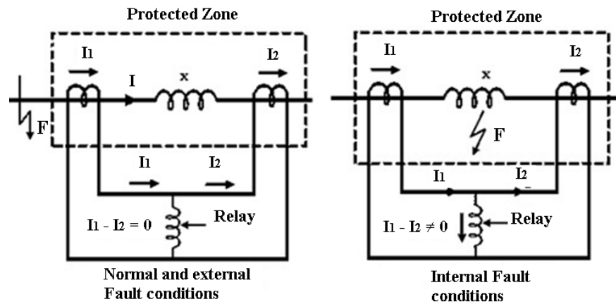
Figure 1. Differential relay working principle.
