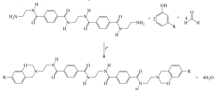
Figure 2. Benzoxazine is synthesized from AET, cardanol and paraformaldehyde.
