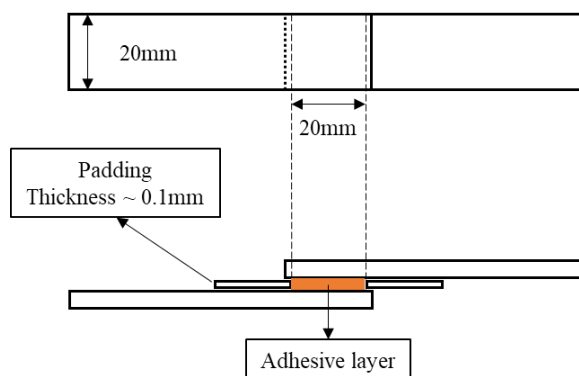
Figure 3. Samples for lap-shear adhesion testing.
