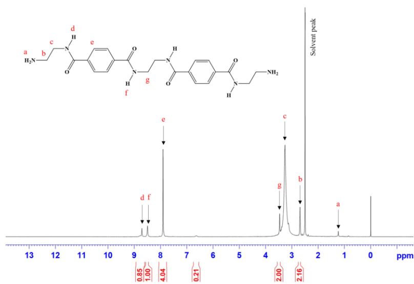
Figure 5. ^1\text{H} -NMR spectra of AET.
