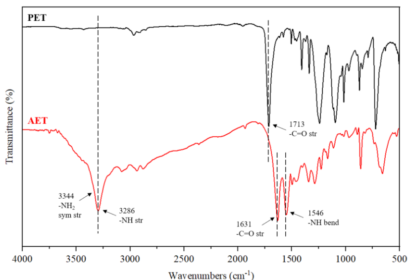
Figure 4. FTIR spectra of PET and AET.
