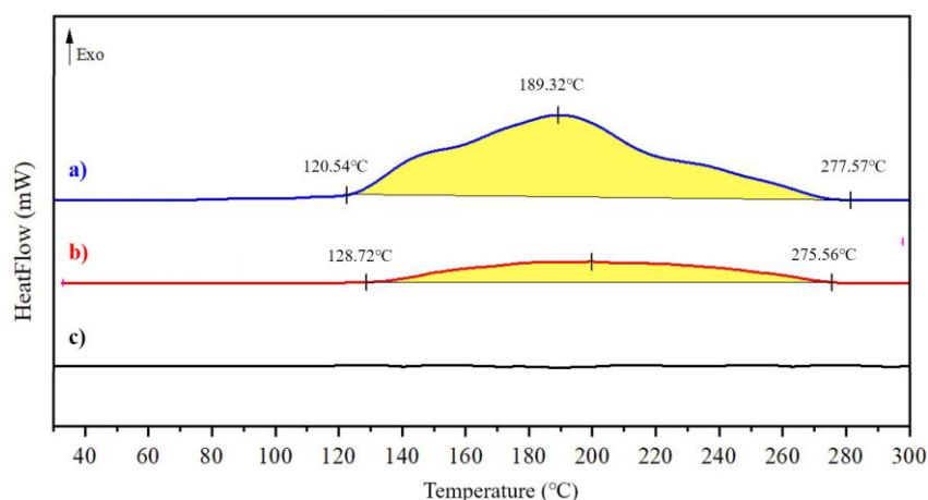
Figure 8. DSC of benzoxazine resin C-AET a) Not cured yet, b) cured 30 min, c) cured 60 min.
