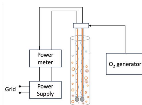
Figure 1. Schematic configuration of the water plasma system.
