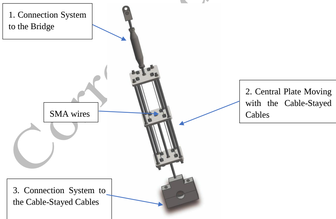
Figure 1. Overall concept of a two-stage damper using shape memory alloy materials.
